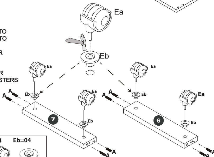
Caster and insert
